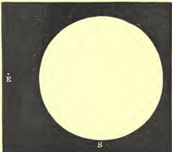
Fig. 4.—Comparative sizes of Earth and Sun.
